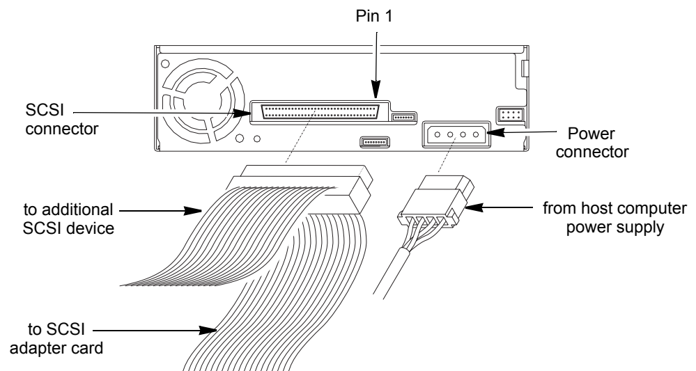
Figure 2-3 Connecting the SCSI cable and power cable (another device is the last device on the bus)
